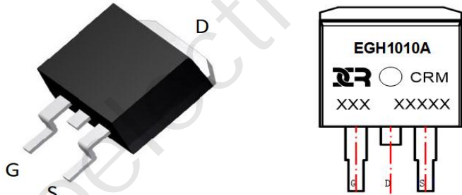
Marking and Pin Assignment
